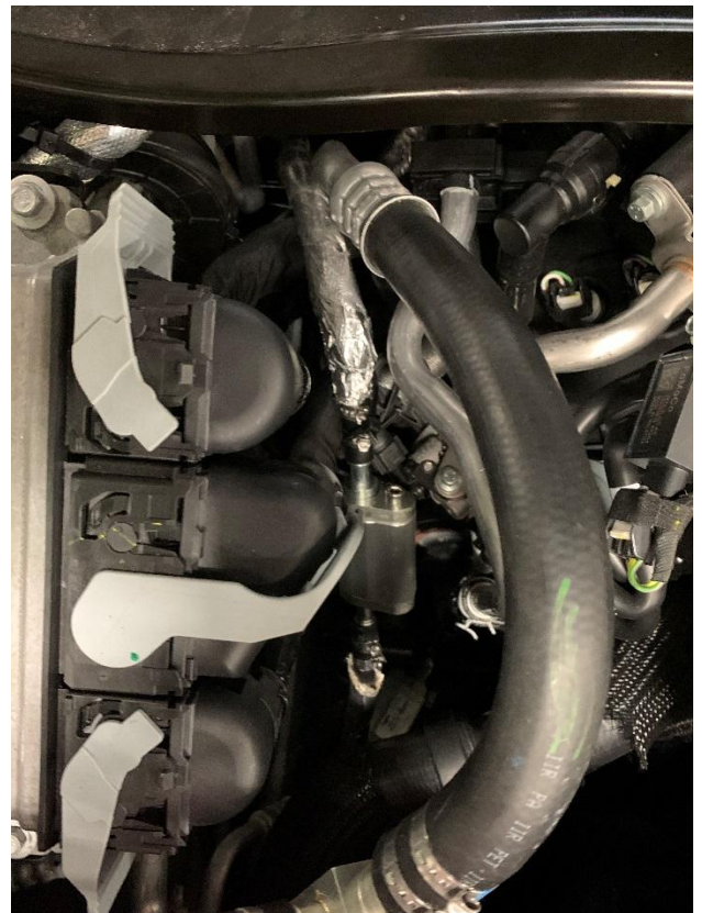
Figure 1.14: Completed Suction and Discharge Lines
