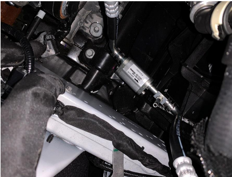
Figure 1.14: Completed Suction and Discharge Lines
