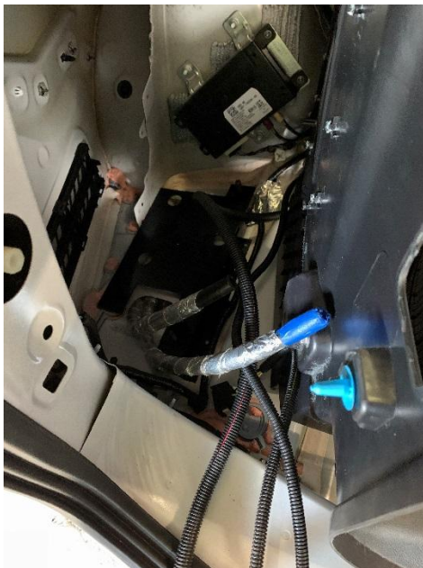
Figure 1.8: Location of Hose Routing Hole
