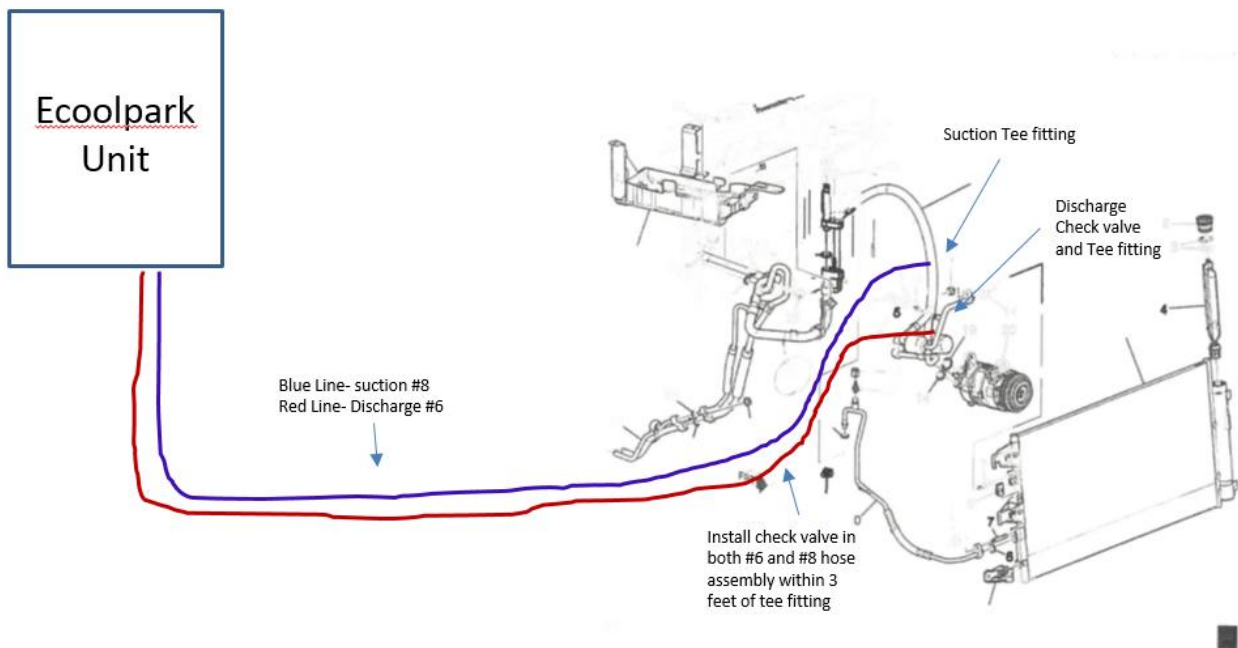
Figure 1.16: Hose Routing Schematic Example
