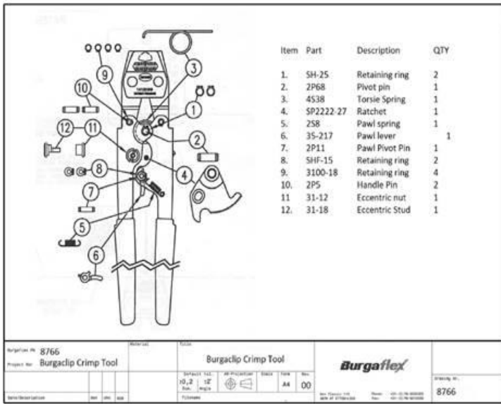
Figure 1.17: Ratcheting Refrigerant Hose Crimpers
