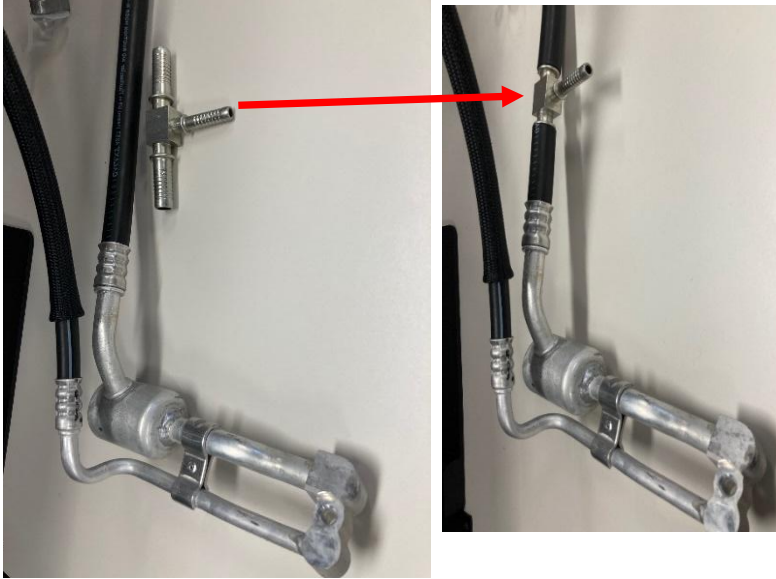
Figure 1.11: Suction Line Alteration on 2021-2022 Tahoe
