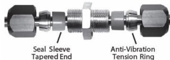
Figure 1.18: Compression T
