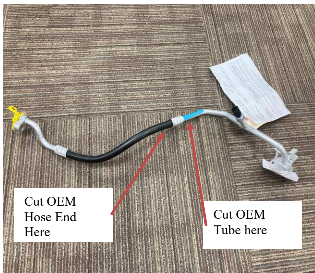
Figure 1.10: Discharge Line Removed
