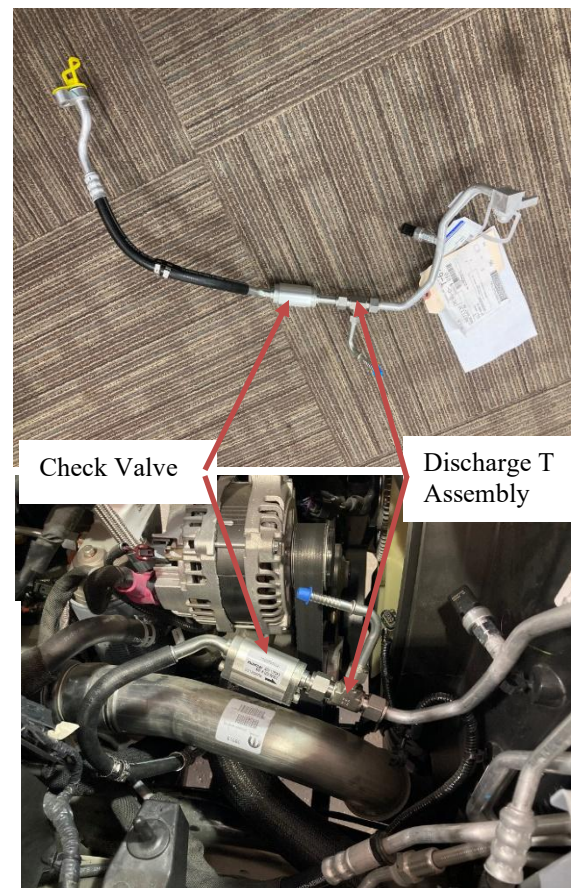
Figure 1.11: Discharge Line Installed
