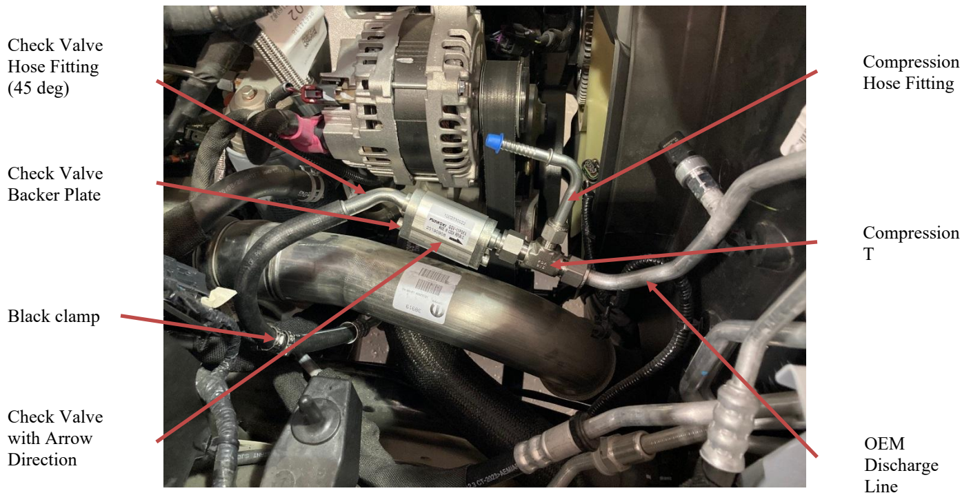
Figure 1.14: Finished A/C Hose Alteration
