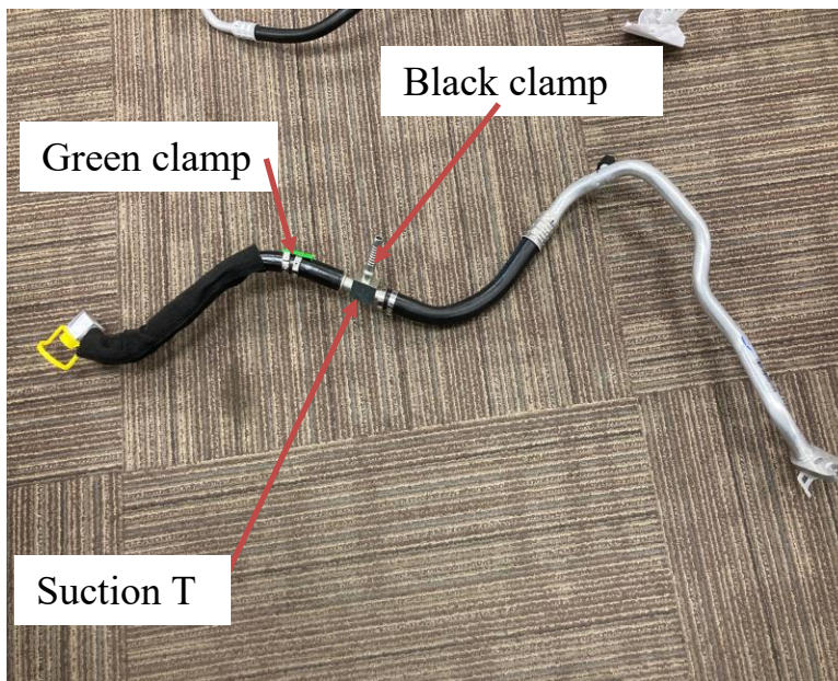
Figure 1.9: Suction Line Removed
