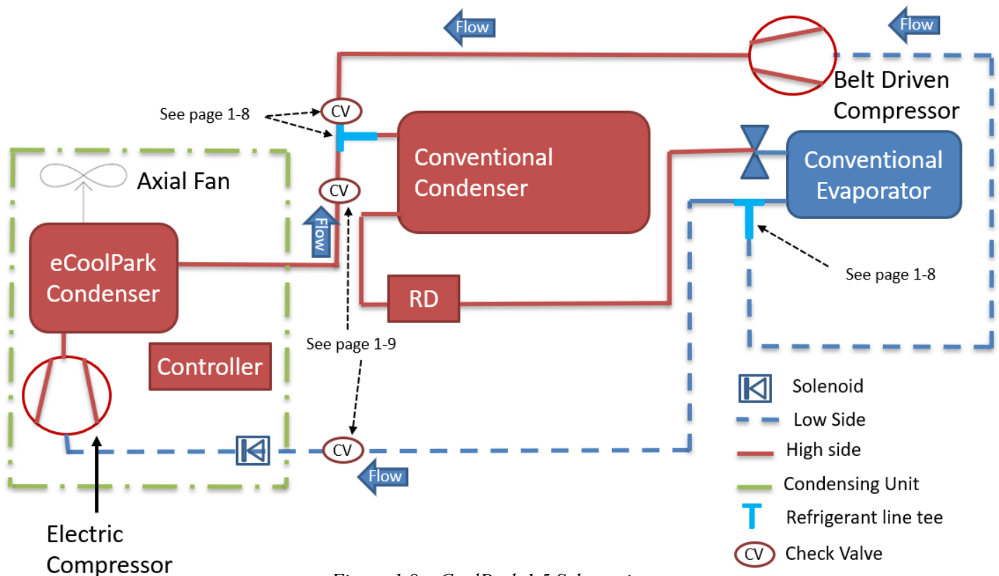
Figure 1.8: eCoolPark 1.5 Schematic
