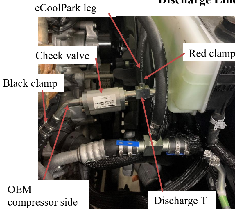
Figure 1.10: Discharge T In Vehicle
