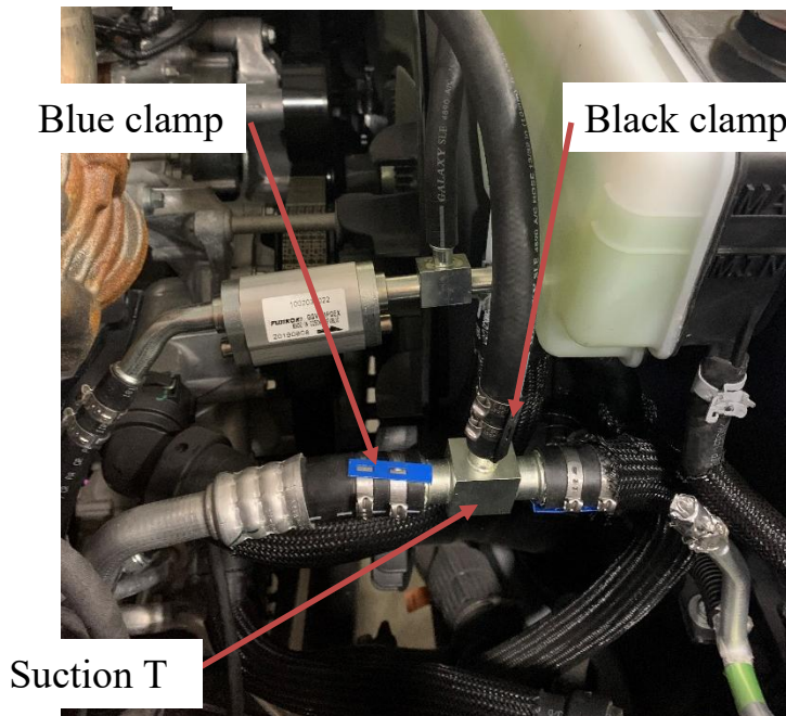
Figure 1.9: Suction T In Vehicle
