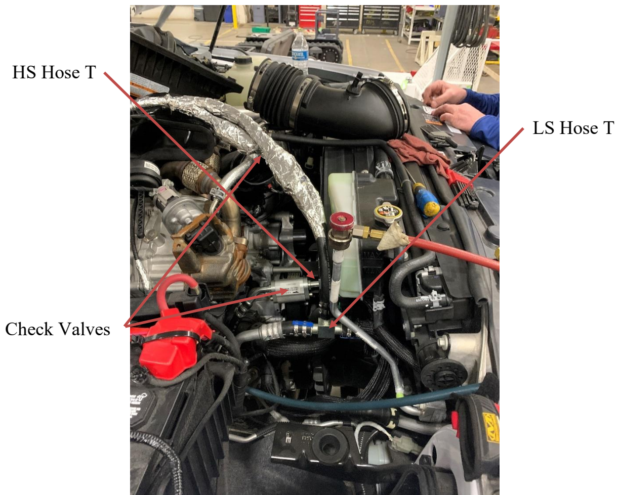
Figure 1.13: Finished A/C Hose Alteration
