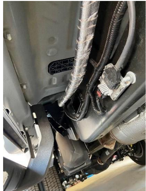
Figure 1.7: Hoses Routed Under Vehicle
