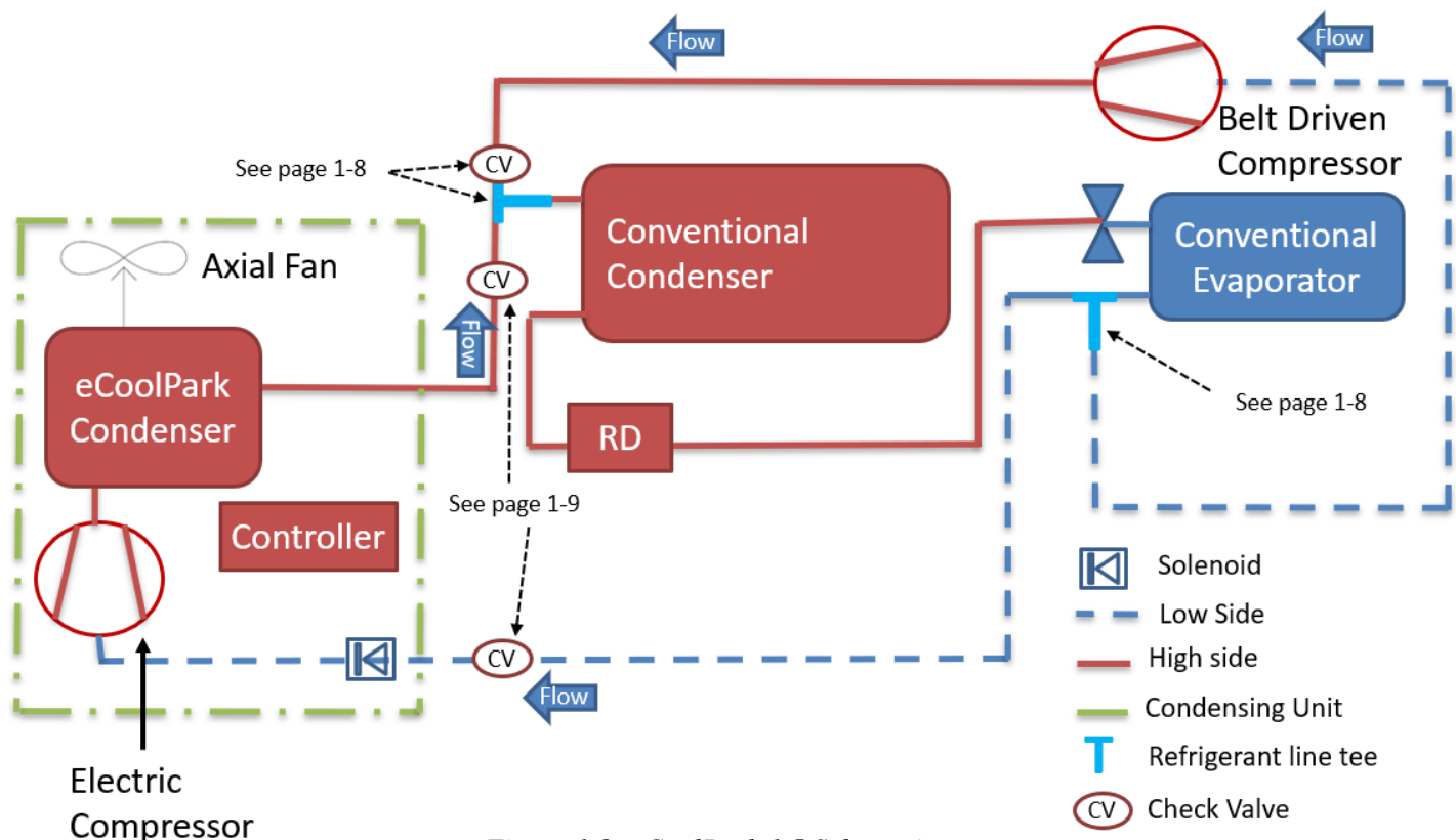
Figure 1.8: eCoolPark 1.5 Schematic
