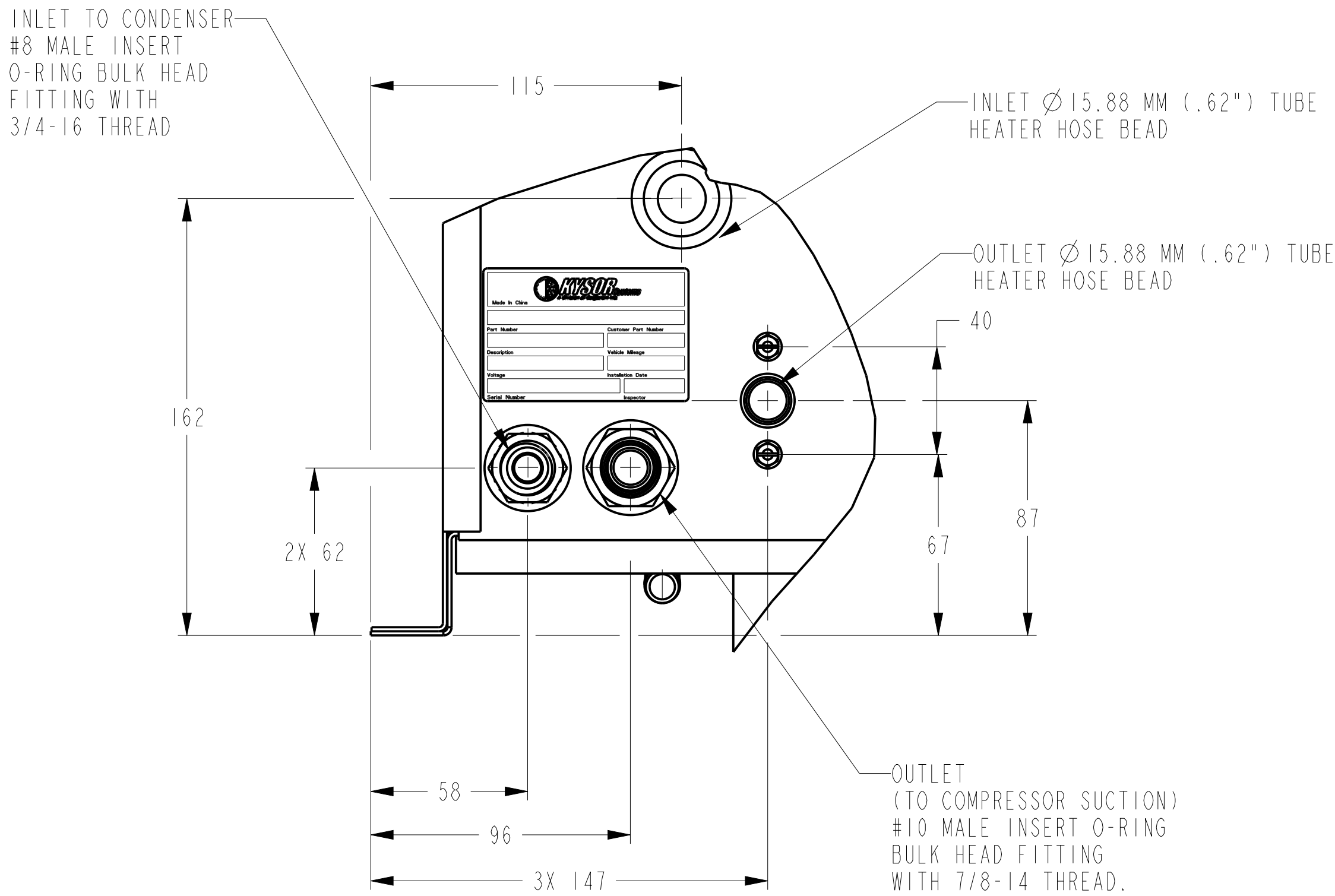
DETAIL A
