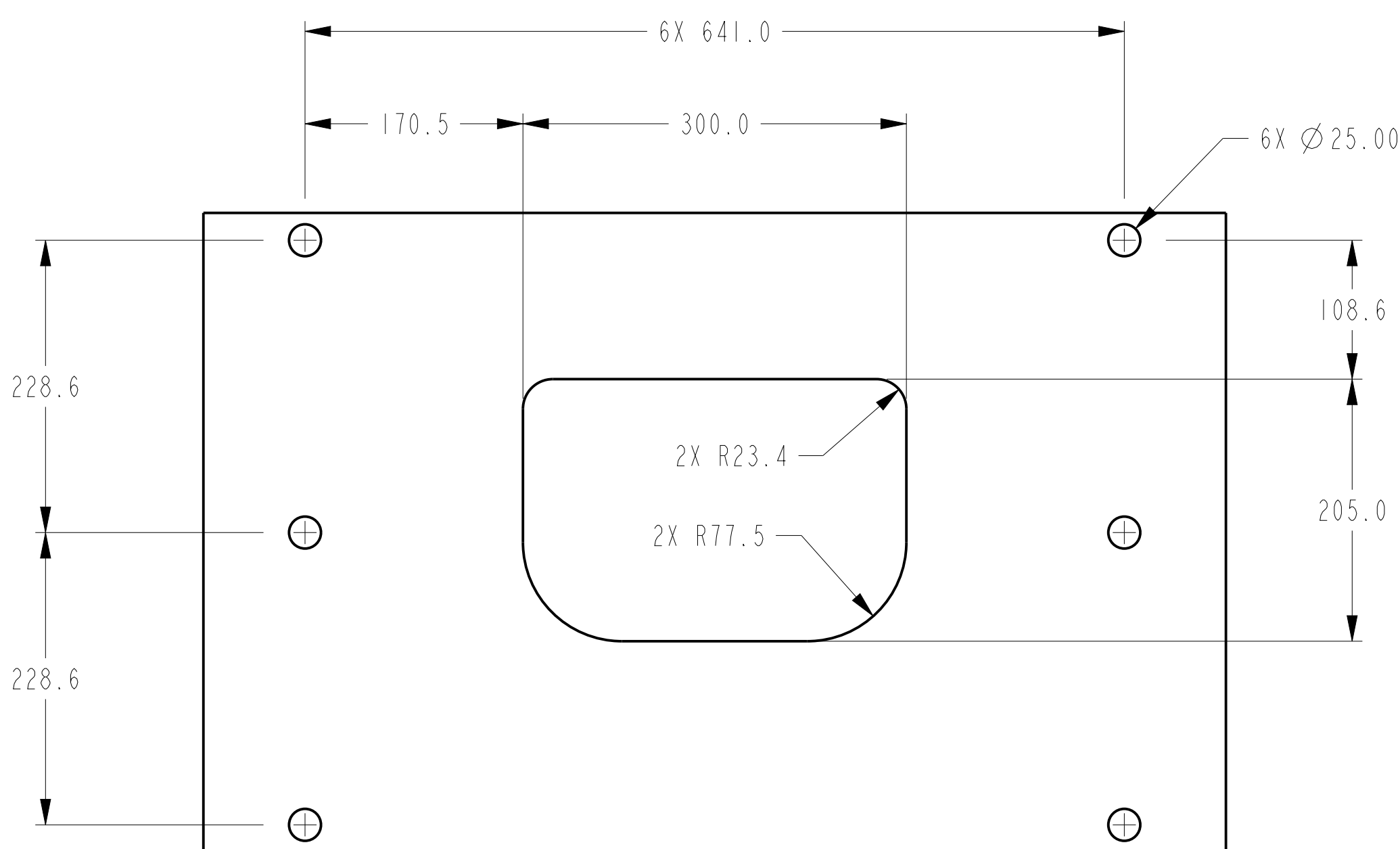
MOUNTING TEMPLATE #342125 ROOF CUT OUT DIMENSIONS
